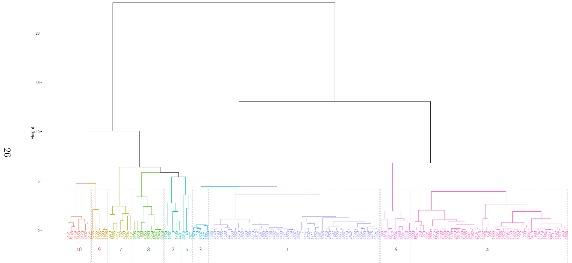
Figure 3: Dendrogram
