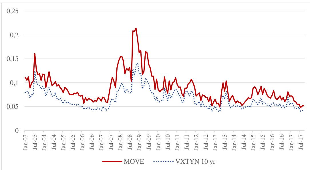
Figure A.2. VXTYN and MOVE: January 2003-September 2017
