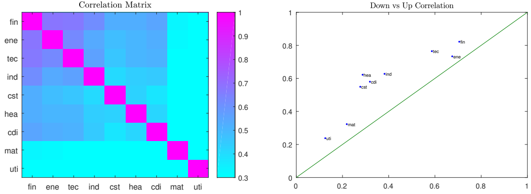
Figure 4.4: Implied Correlations for the Nine Sectors on September 8, 2008. The left panel shows the correlation matrix. The right panel shows the implied down correlation \rho_{i,S}^{d,Q} versus up correlation \rho_{i,S}^{u,Q} . Also shown is the 45-degree line.
