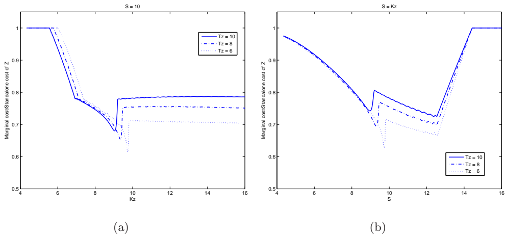
Figure 9: Ratio of incremental cost of new grant Z in portfolio with existing option Y , as a proportion of stand-alone cost of Z for different T_Z s. Left graph vs K_Z with S = 10 , right graph vs S for ATM option grant of Z . Option Y has K_Y = 10 , T_Y = 5 . Parameter values: \gamma = 0.2 , r = 0.05 , q = 0 , \eta = 0.2 , \rho = 0 .
