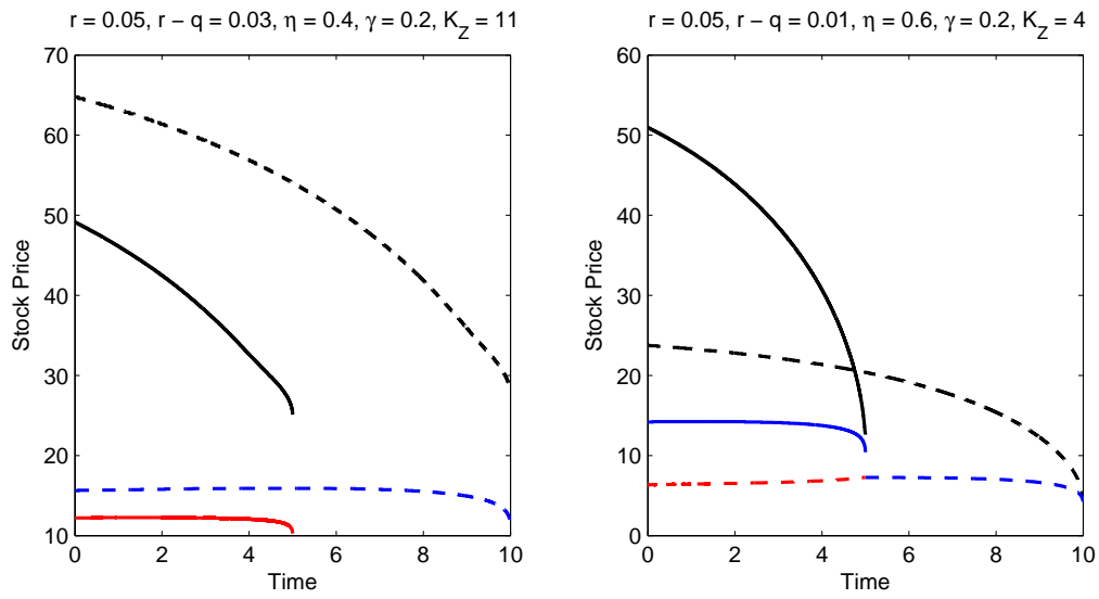
Figure 2: Option Y has K_Y = 10, T_Y = 5 ; option Z has T_Z = 10 . In the left panel, K_Z = 11 ; in the right panel K_Z = 4 . Parameter values where not stated: \rho = 0 .
