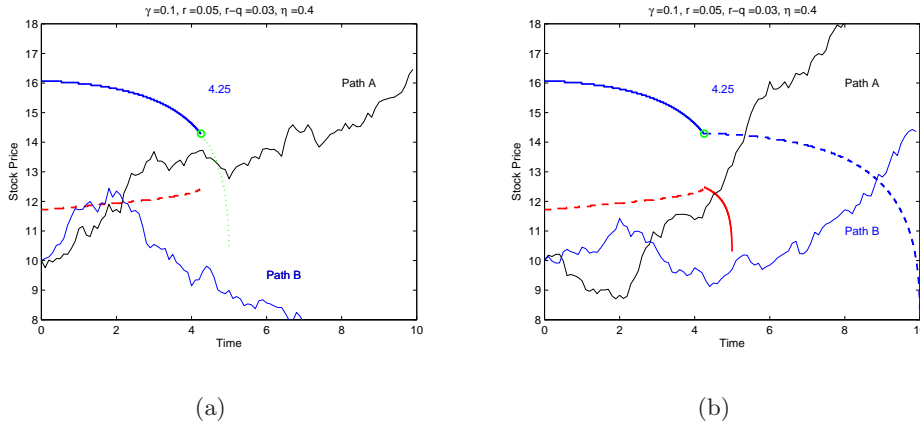
Figure 4: Option Y has K_Y = 10, T_Y = 5 ; option Z has K_Z = 8, T_Y = 10 . Parameter values: \gamma = 0.1, r = 0.05, q = 0.02, \eta = 0.4, \rho = 0 .
