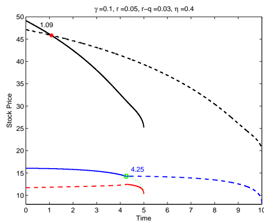
Figure 3: Option Y has K_Y = 10, T_Y = 5 ; option Z has K_Z = 8, T_Z = 10 . Parameter values: \gamma = 0.1, r = 0.05, q = 0.02, \eta = 0.4, \rho = 0
