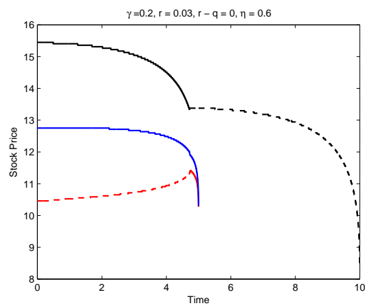
Figure 10: Portfolio with Two options with K_Y = 10, T_Y = 5 and one option with K_Z = 8, T_Z = 10 . Parameter values: \gamma = 0.2, r = 0.03, q = 0.03, \eta = 0.6, \rho = 0 .
