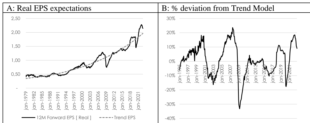
Figure 4: Real EPS and deviation from trend
